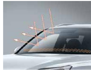
Solar control glass and wiper deicer
